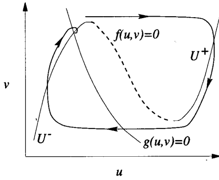
FIG. 2. Sketch of phase plane of the local kinetics of Eqs. (1) and (2), with n = n_0 . The solid portions U^\pm of the f -nullcline are stable, in the sense that nearby trajectories remain close. The dashed portion is unstable.
